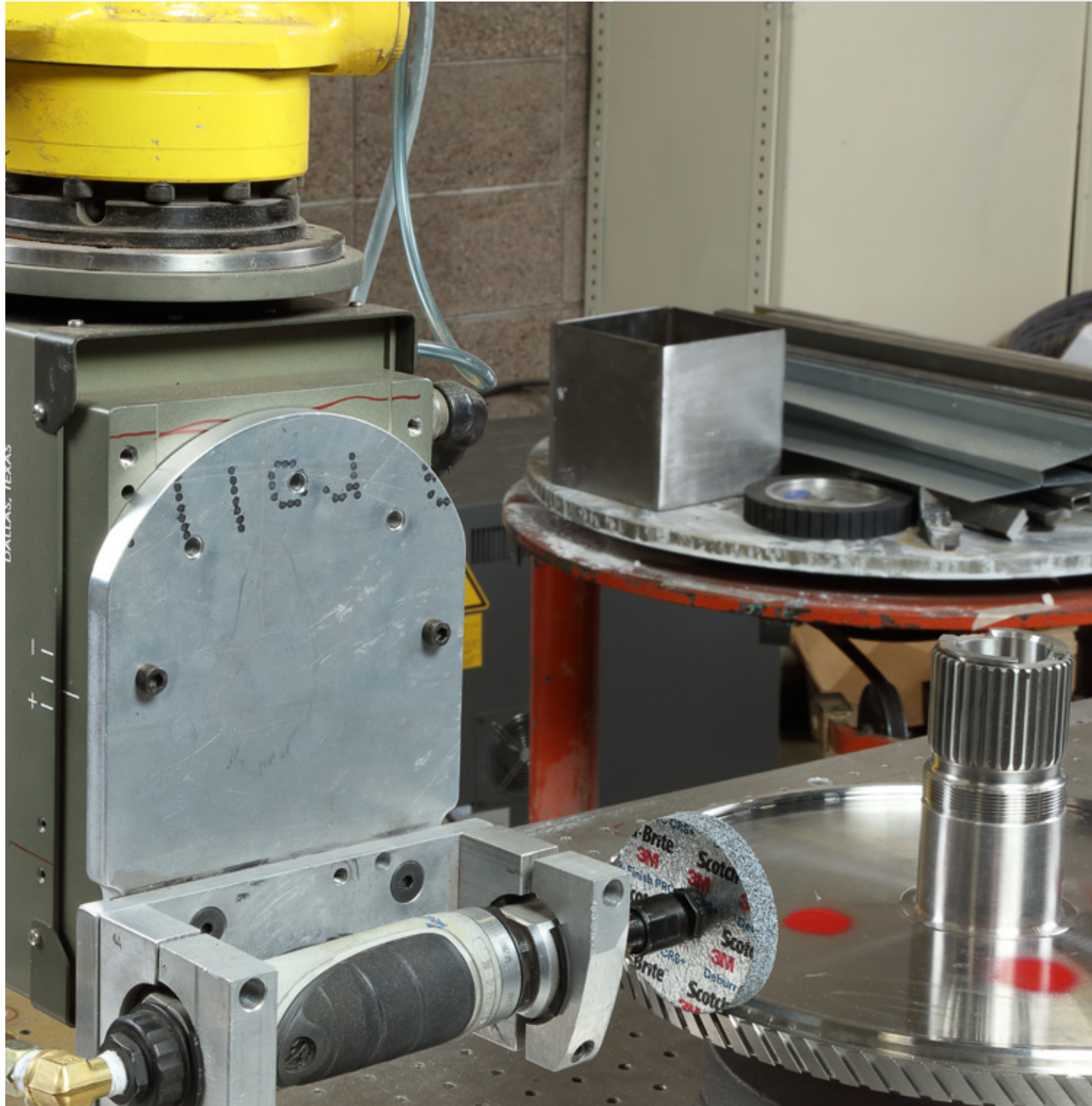
Deburring with a PushCorp Inc. force control device and a Scotch-Brite deburr and finish Pro wheel.
